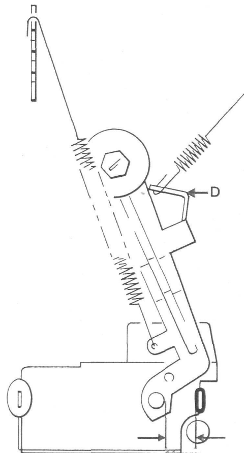
Left tape tension arm
