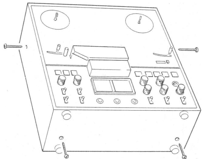
Cabinet screws
