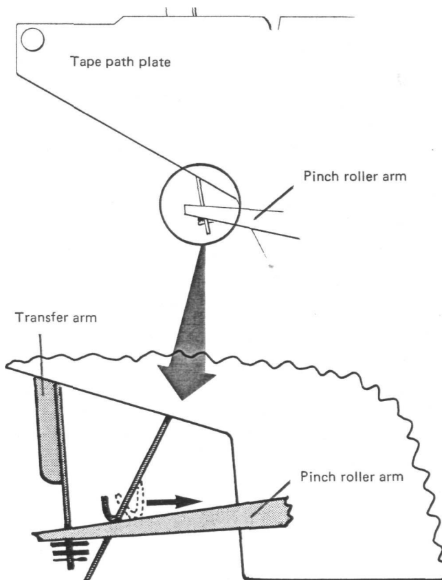
Adjusting the transfer arm
