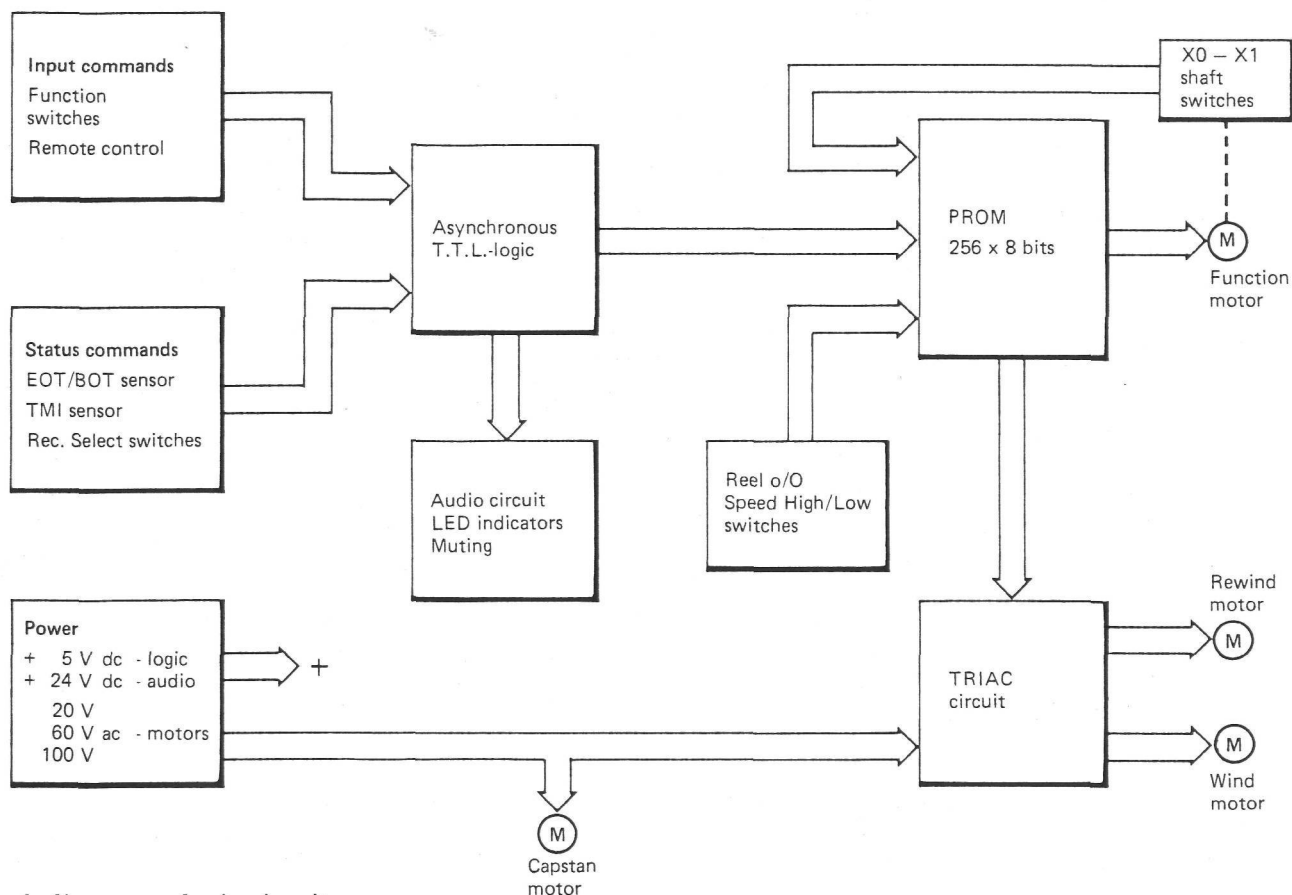
Block diagram – logic circuits
