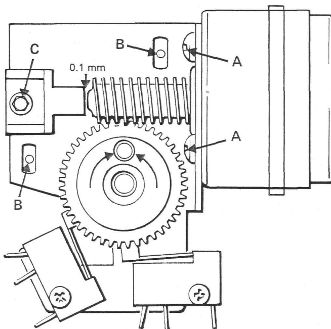
Adjusting the worm-gear motor
