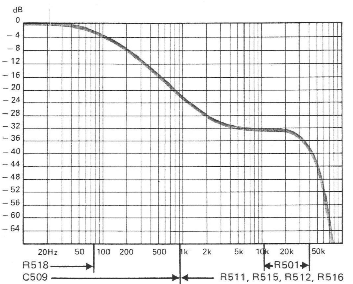
Playback correction curve 7 1/2 ips
