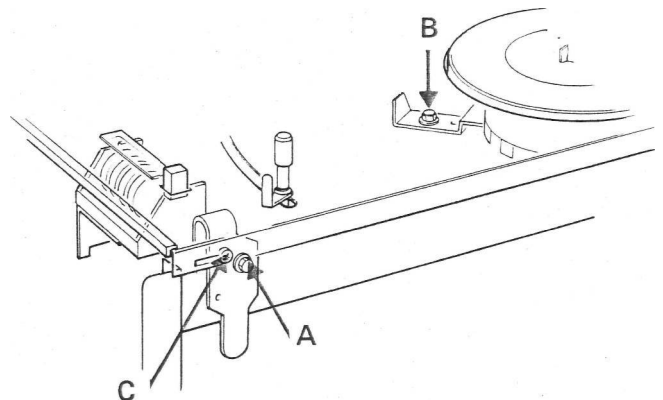
The sensor arm and the counter screws
