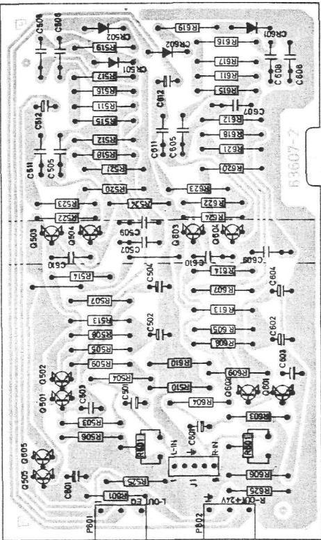
Playback amplifier board (solder side)
