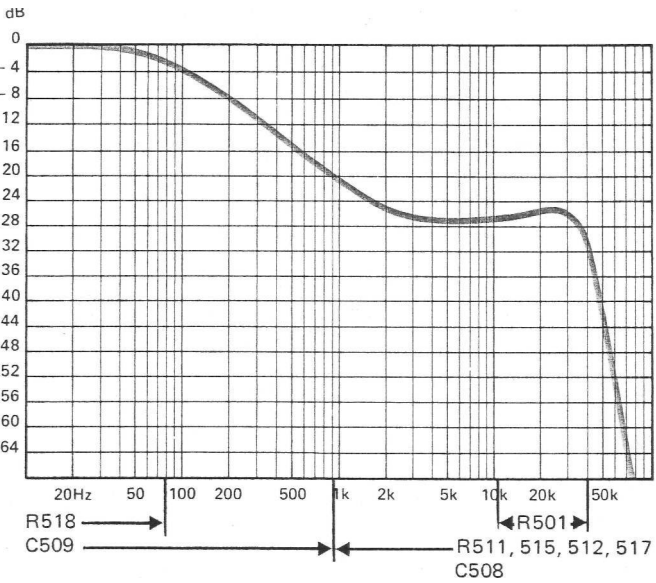
Playback correction curve 3 3/4 ips
