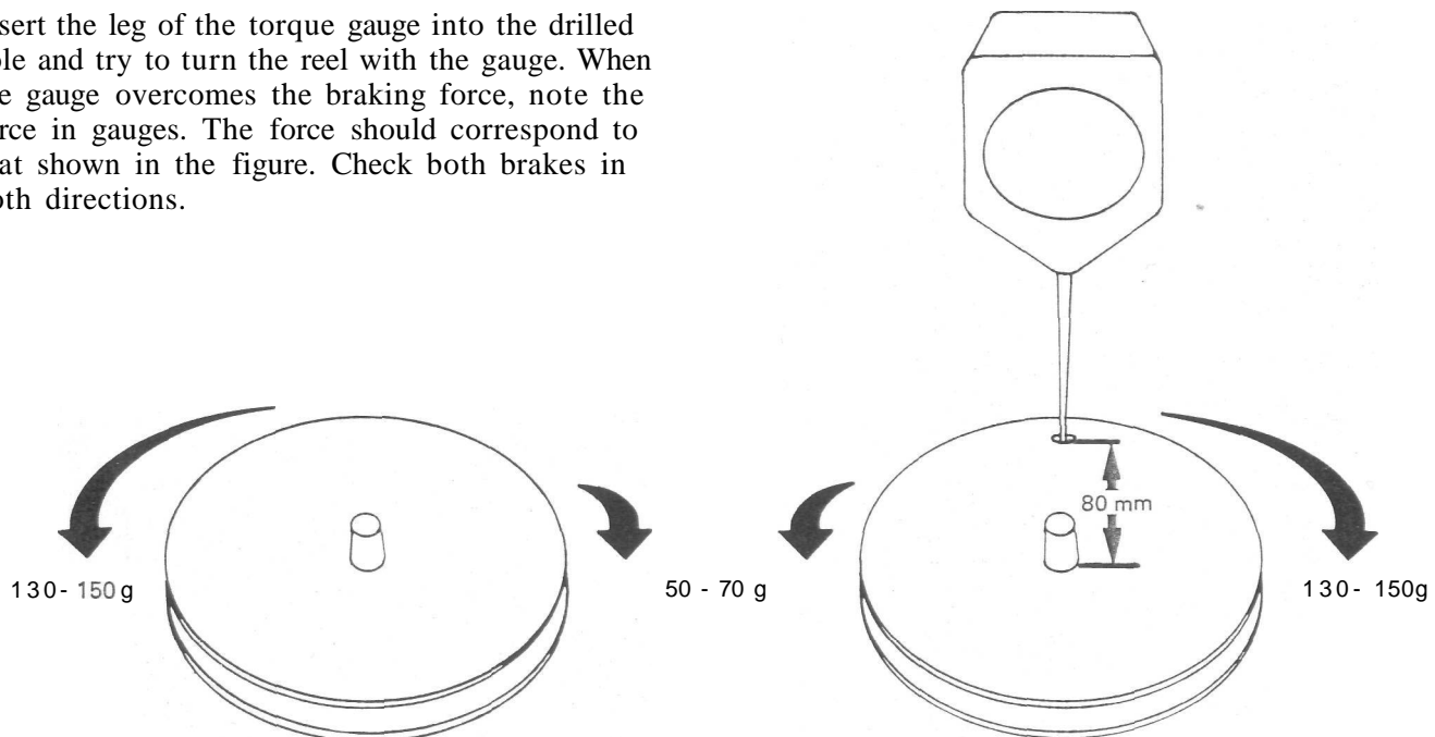
Checking the braking force
