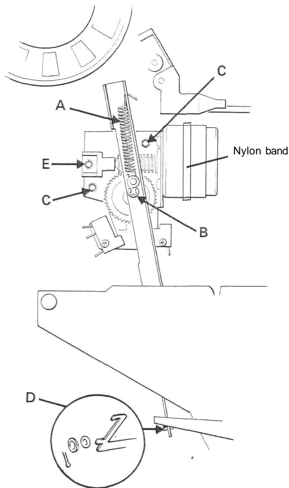
Dismantling the worm-gear motor
