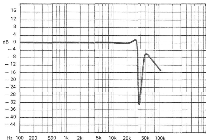
38 kHz trap curve
