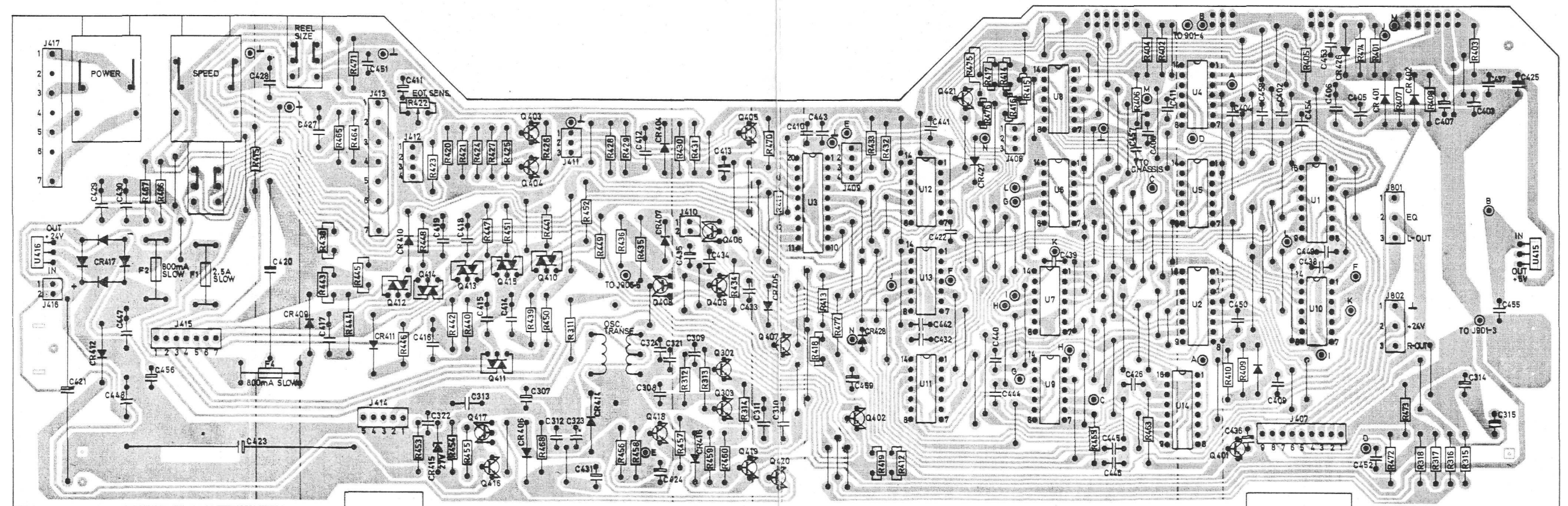
LOGIC BOARD, SOLDER SIDE
