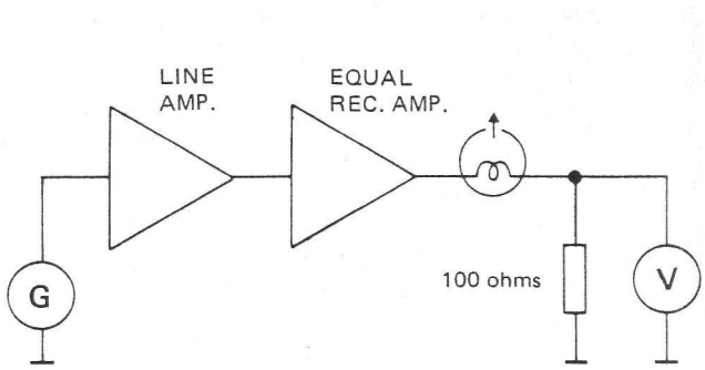
Checking the record curve
